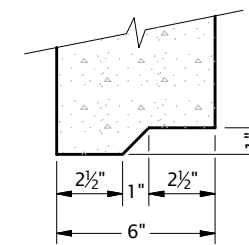
KEYWAY DETAIL
