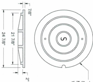
TWO HOLE 'S' COVER STANDARD NO VENT HOLES IN WATERTIGHT COVERS
